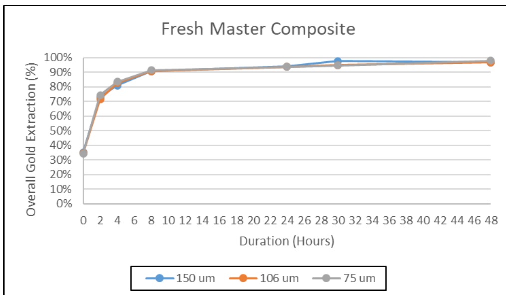
Figure 5 Gravity Gold + Cyanide Leach Curves for Fresh composites
