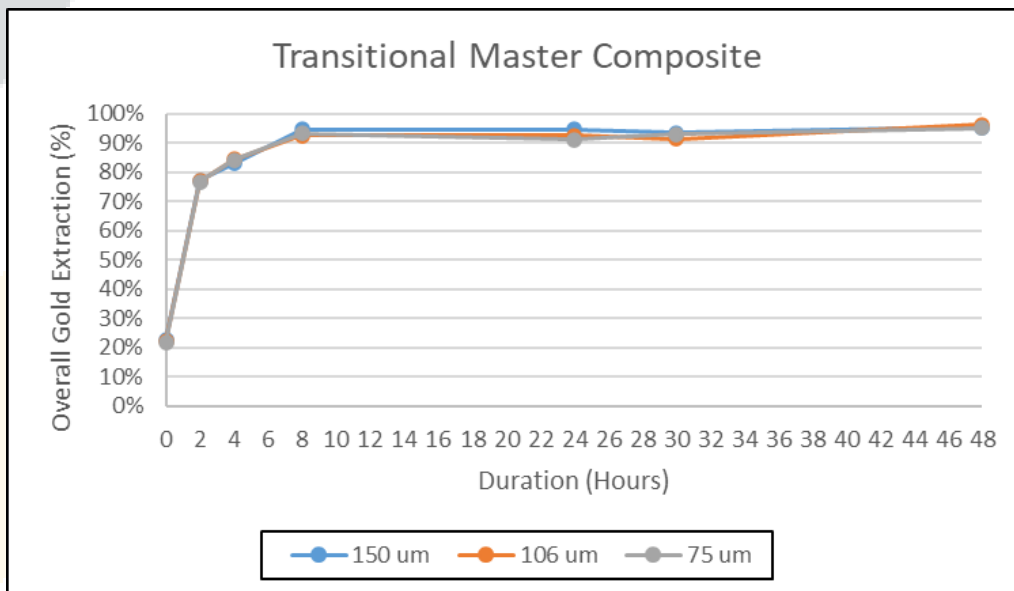
Figure 4 Gravity Gold + Cyanide Leach Curves for Transitional composites
