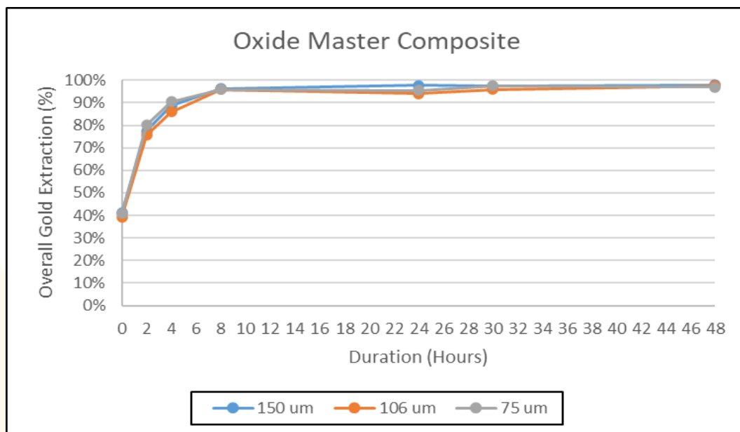
Figure 3 Gravity Gold + Cyanide Leach Curve for Oxide composites
