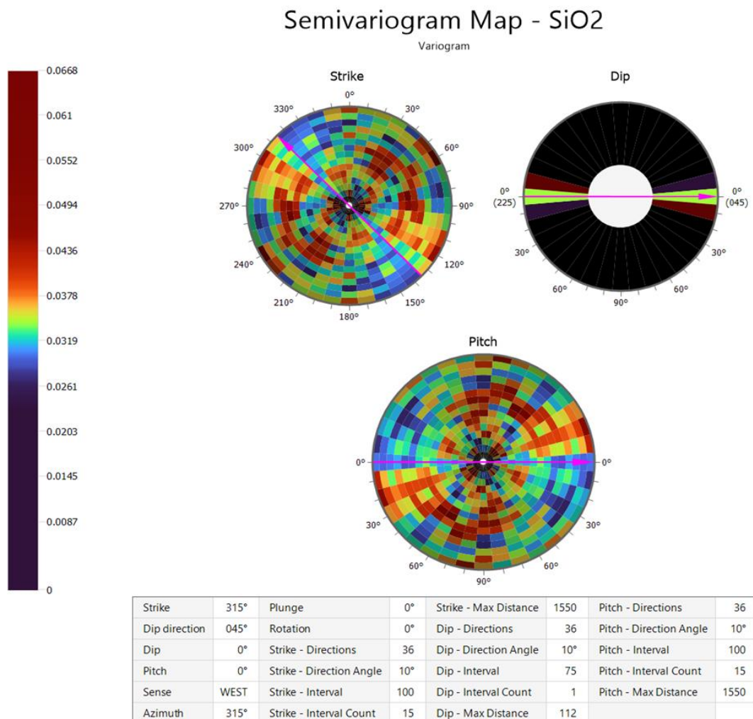
Figure 6: Semivariogram Map - SiO 2
